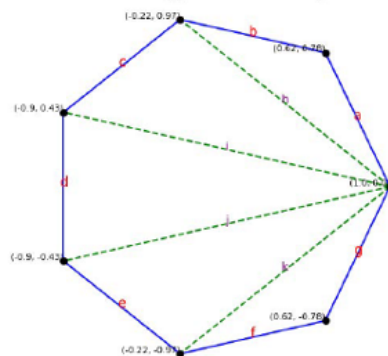
7-sided Polygon with Minimal Diagonals
