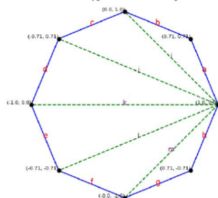
8-sided Polygon with Minimal Diagonals
