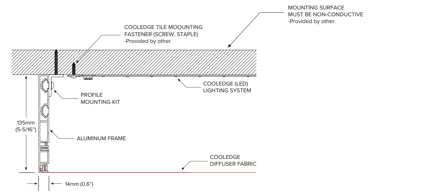
X-Section
